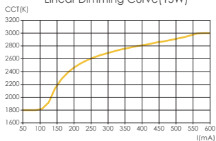
Linear Dimming Curve(15W)
